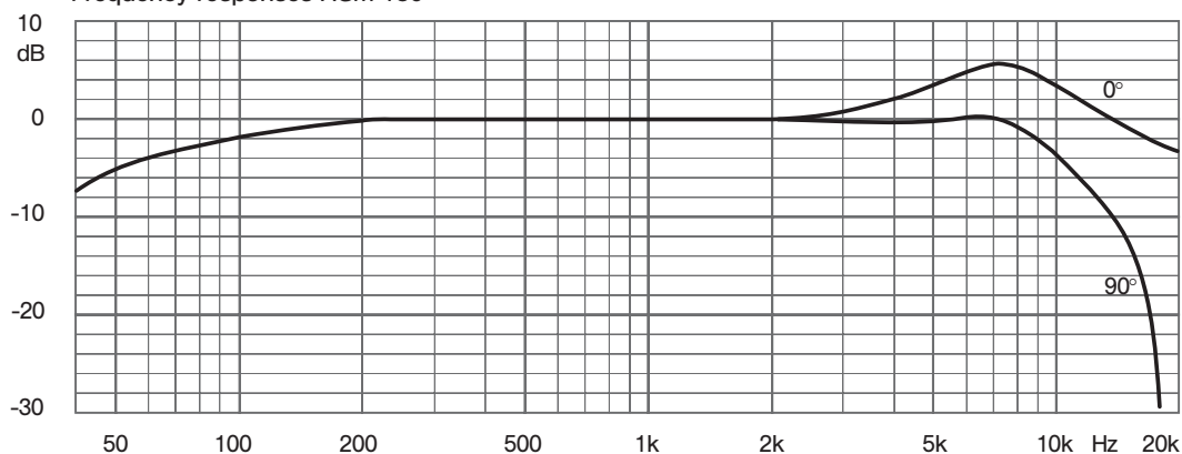
Frequency responses HSM 180
