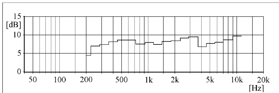
Directivity index
