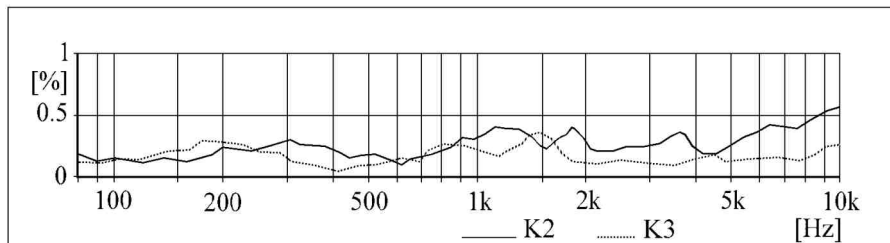
Total harmonic distortion P_A = 96 dB
